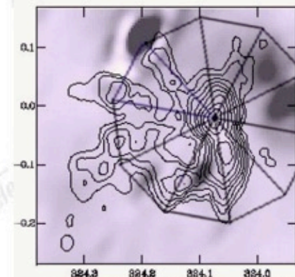
Great Attractor hub to many superclusters spread along seven arms of decagon-helix
