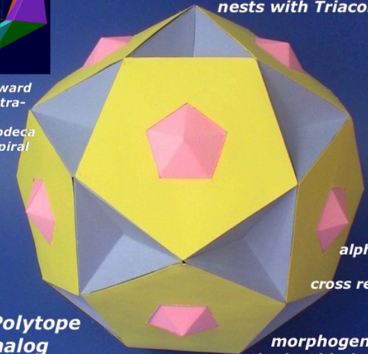
Icosidodeca shell of 120 Cell nests with Triaconta [pink]
