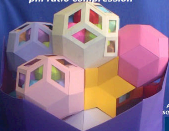
144 Triaconta nest around Rhombic Hexeconta any or all Triaconta can implode through their own centre or main heart centre
