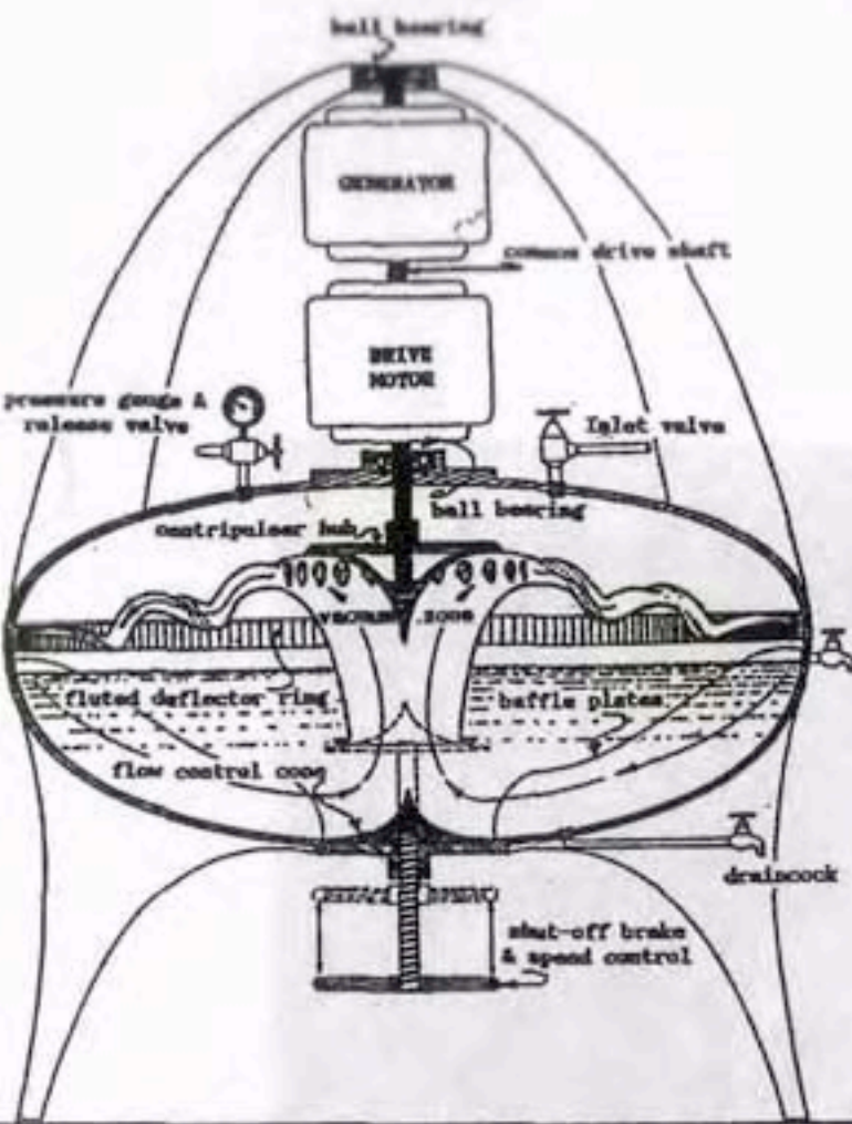
SECTION THRO TORNADO GENERATOR
